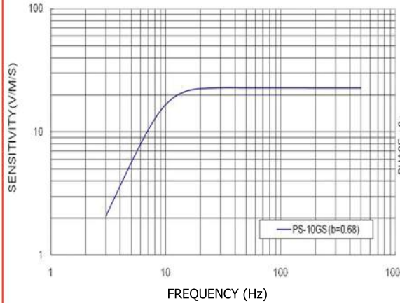
PS-10 GS AMPLITUDE FREQUENCY CURVE
