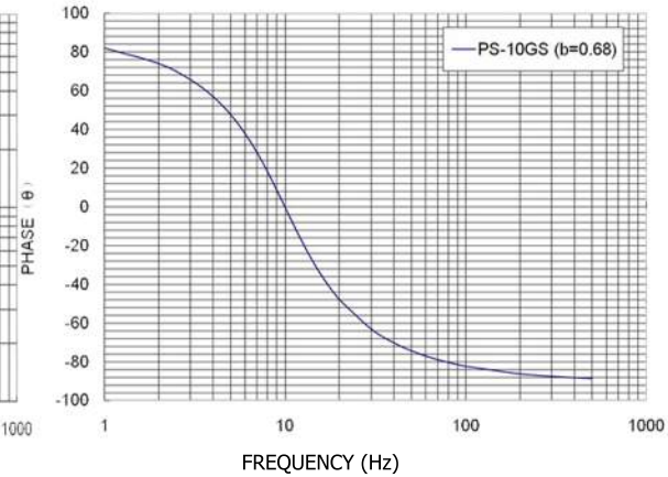
PS-10 GS PHASE FREQUENCY CURVE
