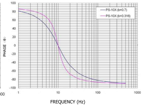
PS-10XS PHASE FREQUENCY CURVE
