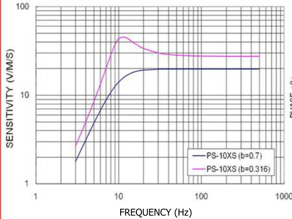
PS-10XS AMPLITUDE FREQUENCY CURVE
