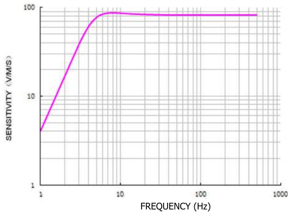
PS-4.5 B AMPLITUDE FREQUENCY CURVE
