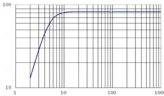
PS-5R AMPLITUDE FREQUENCY CURVE
