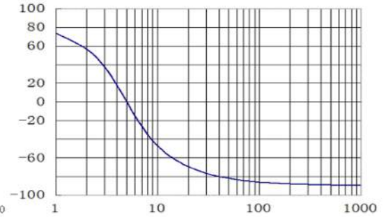
PS-5R PHASE FREQUENCY CURVE
